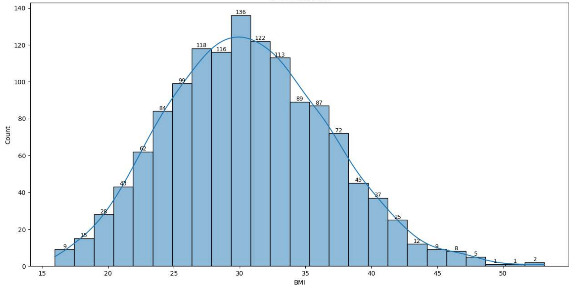
BMI Distribution
